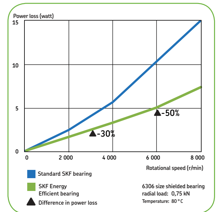
Power loss simulation results showing energy savings of SKF Energy Efficient deep groove ball bearings compared to standard SKF bearings. Energy savings compared to other manufacturers' bearings can be even more dramatic.
